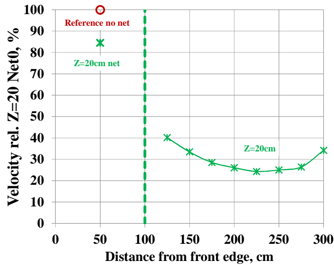
Figure 8. Effect of wind breaking net on the air velocities 20 cm above the center line of the wind table in % of the no net velocity.
