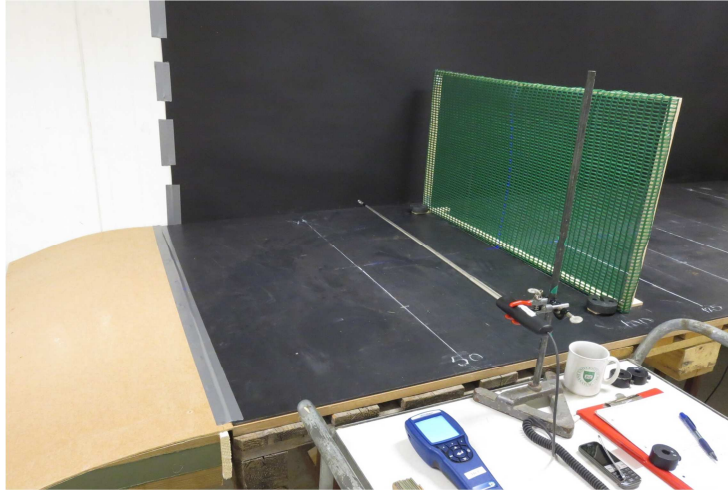
Figure 6. Wind breaking net on the wind table with anemometer in the reference point.
