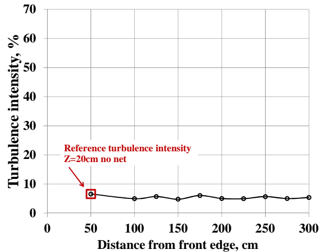
Figure 4. Turbulence intensity 20 cm above the center line of the empty wind table
