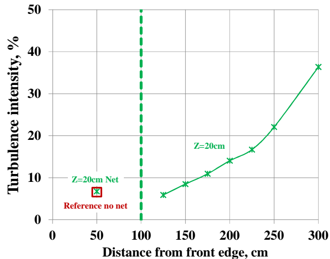
Figure 9. The effect of wind breaking net on the turbulence intensities.
