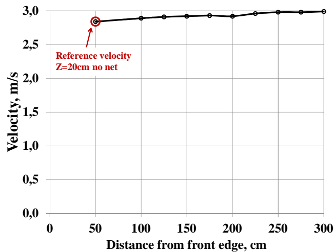
Figure 3. Air velocities 20 cm above the center line of the empty wind table
