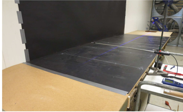
Figure 2. Measurement set-up for calibration of the wind table
