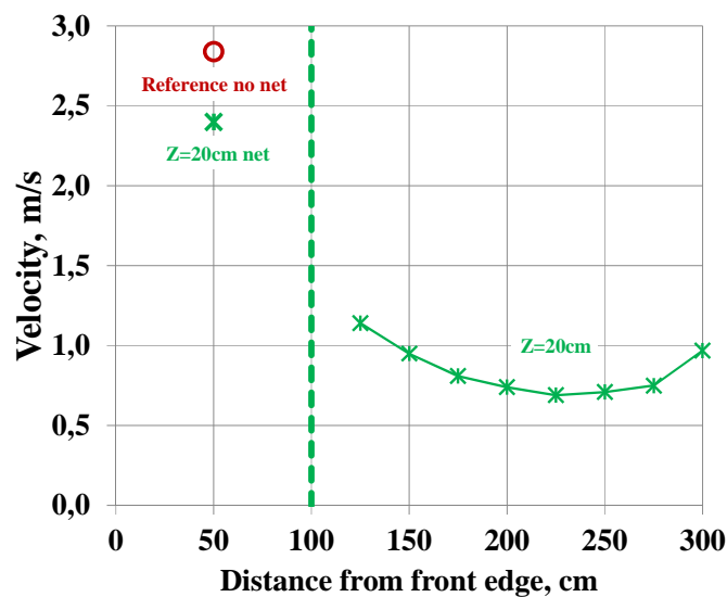
Figure 7. Air velocities 20 cm above the center line of the wind table with wind breaking net
